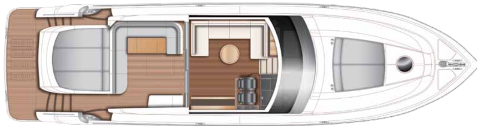
MAIN DECK
