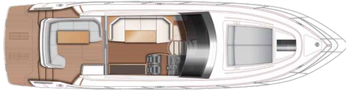
MAIN DECK
